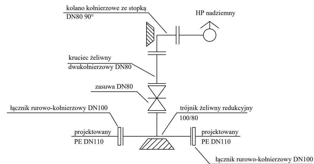
Hydrant HP1
