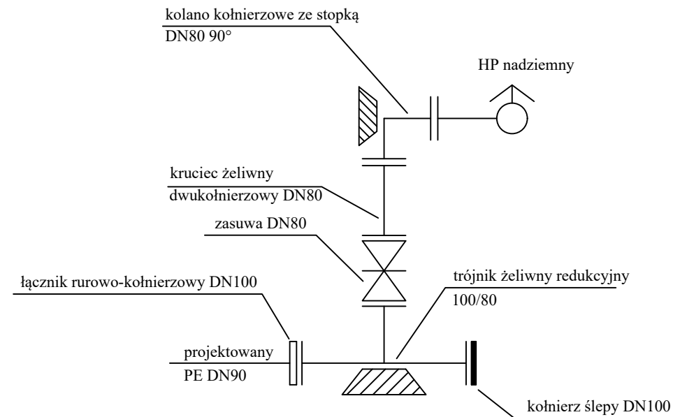
Hydrant HP1
